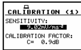
CALIBRATION window during setting the sensitivity smaller than 10.0 \text{ mV} / \text{ms}^{-2}
