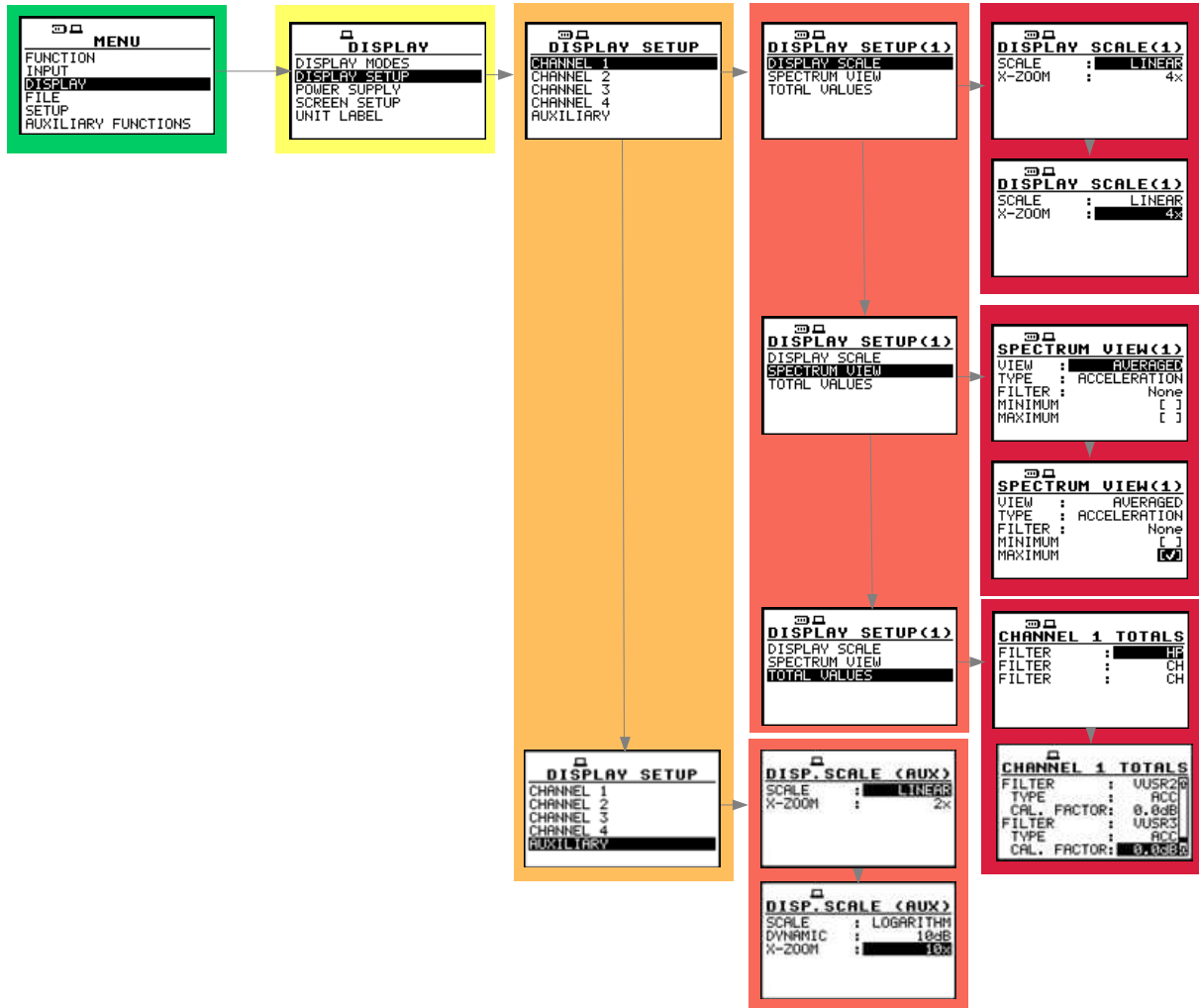
Control diagram of DISPLAY SETUP sub-list in 1/1 OCTAVE and 1/3 OCTAVE analysis
