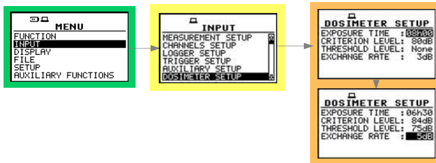
Control diagram of INPUT list in the acoustic DOSIMETER mode
